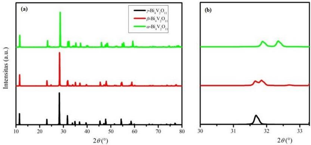
Figure 1 Pattern of X-ray diffraction polymorph oxide BIVOX on angle 2\theta (a) 10-80° and (b) 30-33°. Specific peaks of diffraction polymorph \alpha is on 2\theta 31,7 and 32,32°, specific peaks of polymorph \beta is on 2\theta 31,6 and 31,8°; whereas specific peak of polymorph \gamma is on 2\theta 31,6°. Taken from [12].
